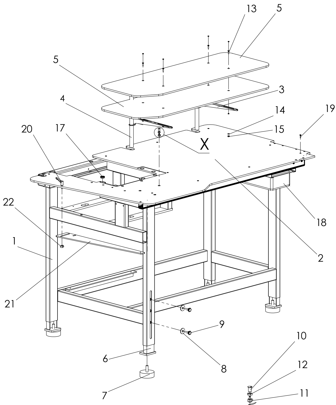
Detail X
